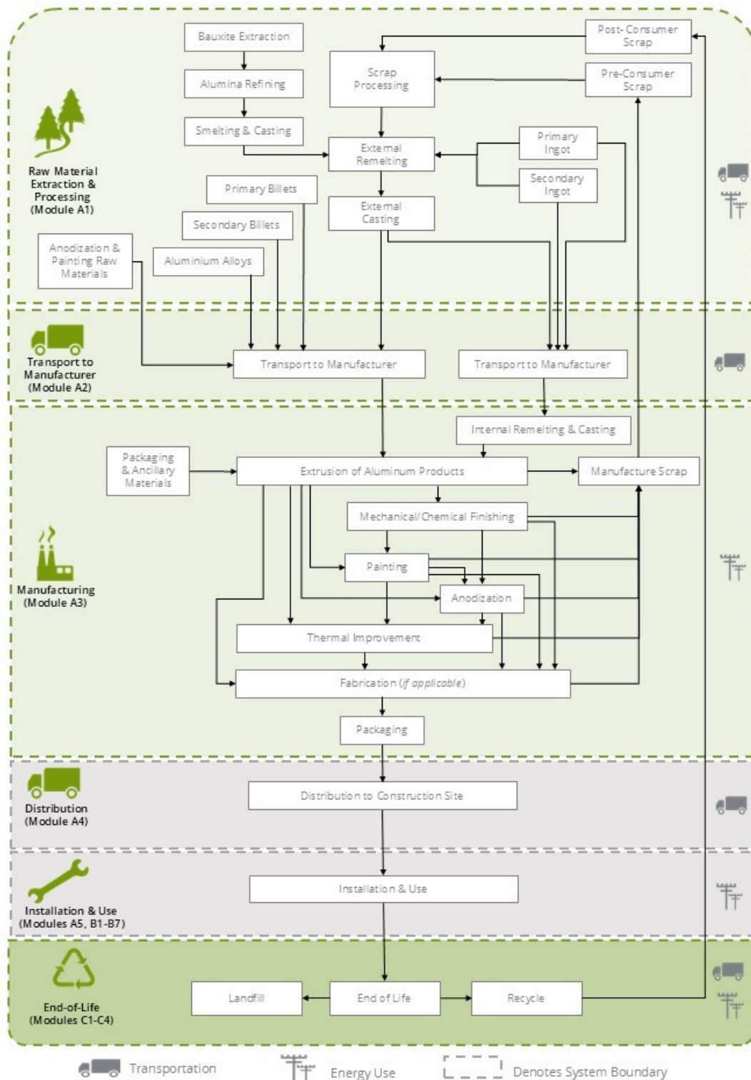
Figure 1. Flow Diagram for the life cycle of the Keymark Corporation Fonda Painted Aluminum Extrusion .
